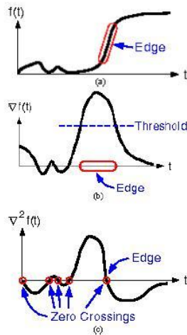
Fig. 1. (a)Original imagesignal (one-dimension); (b)Gradientoftheoriginal imagesignal (firstderivativewithrespecttot); (c)Laplacianoperationonthe originalsinal (second derivative with respect to t)
